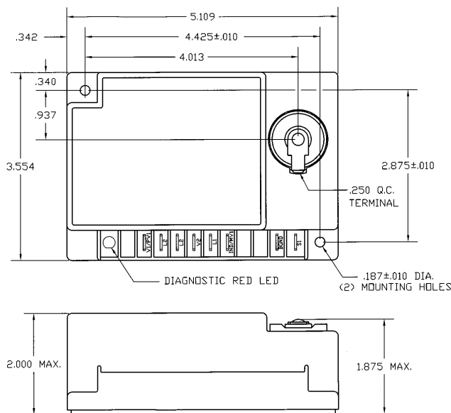
Figure 4. Enclosure
