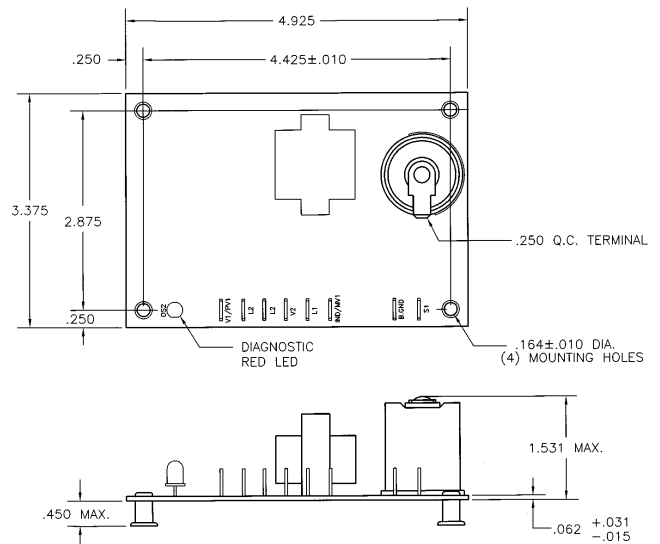
Figure 6. Integral Standoff
