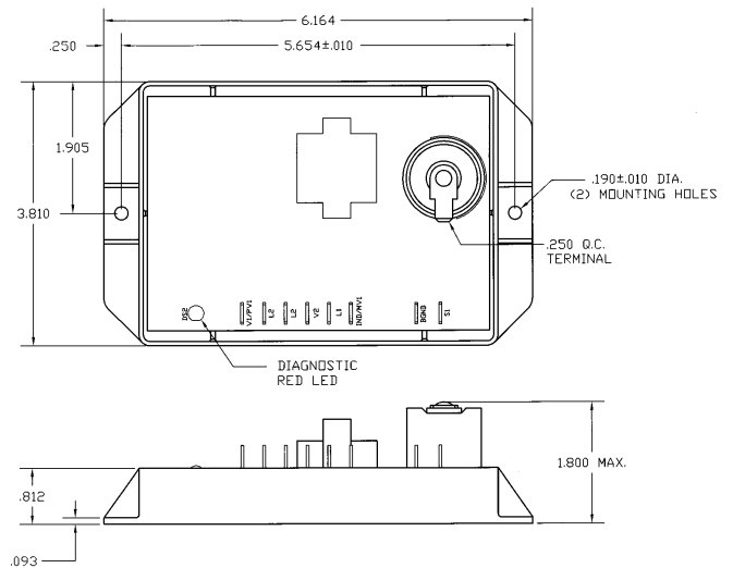
Figure 5. Potted
